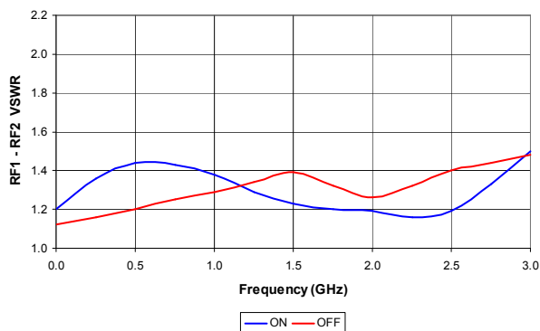
RF1-RF2 VSWR vs. Frequency
